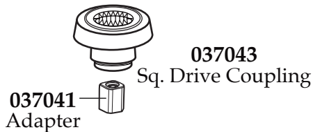
037043 Sq. Drive Coupling 037041 Adapter 503601 Sq. Drive Coupling with Adapter
